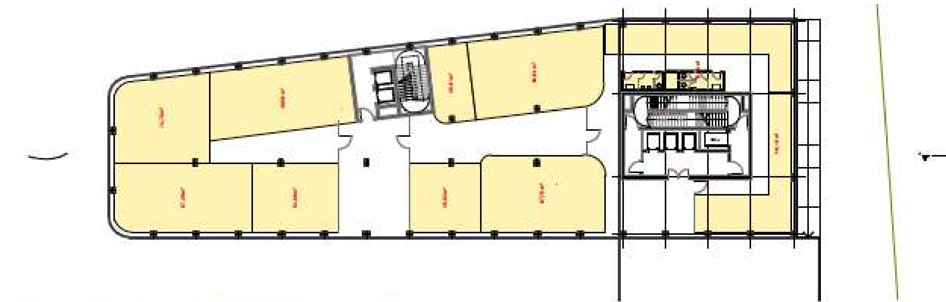
0. ERDGESCHOSS CAMPUS NUF: ca. 692m 2
